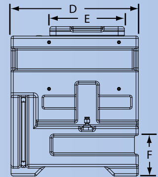
15 Gal. Reservoir
