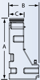
4 Gal. Reservoir
